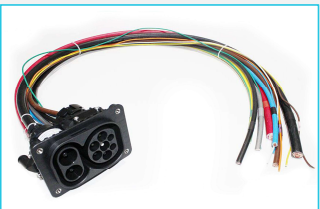
EV Charger Inlet Socket Wire Harness
